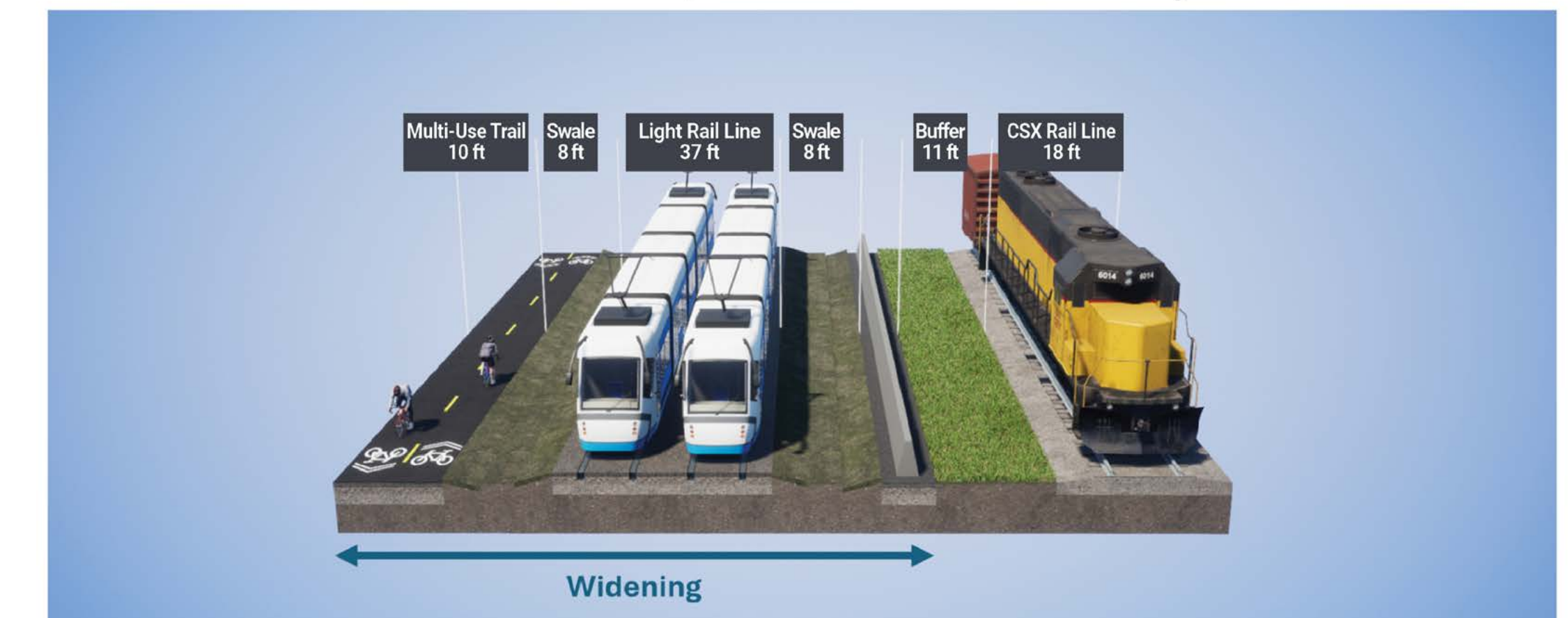
Exclusive Separated LRT Guideway
