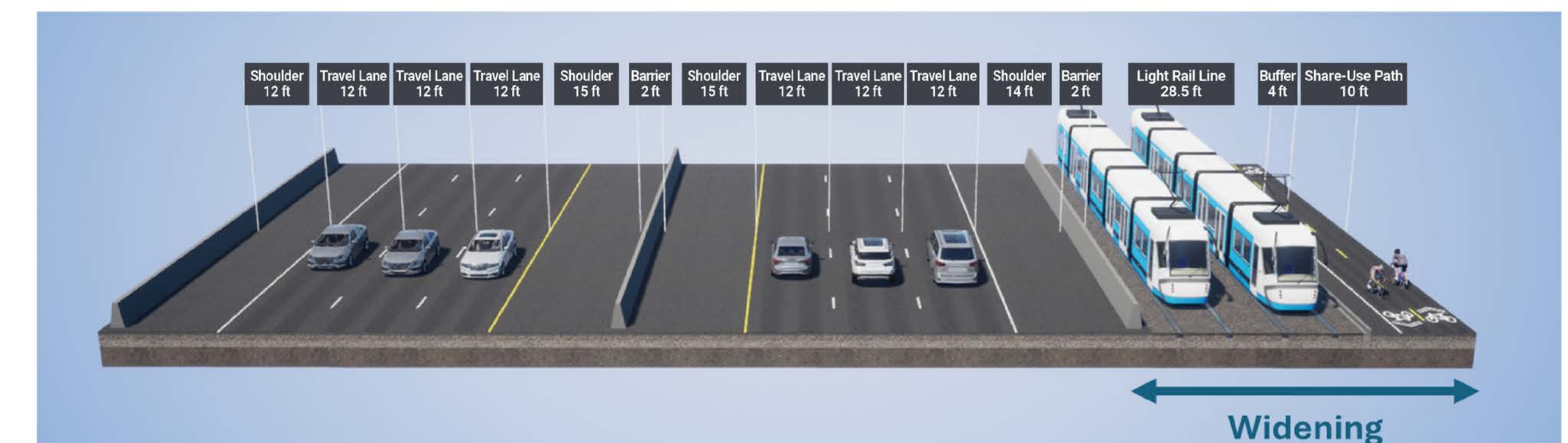
Exclusive Separated LRT Guideway
